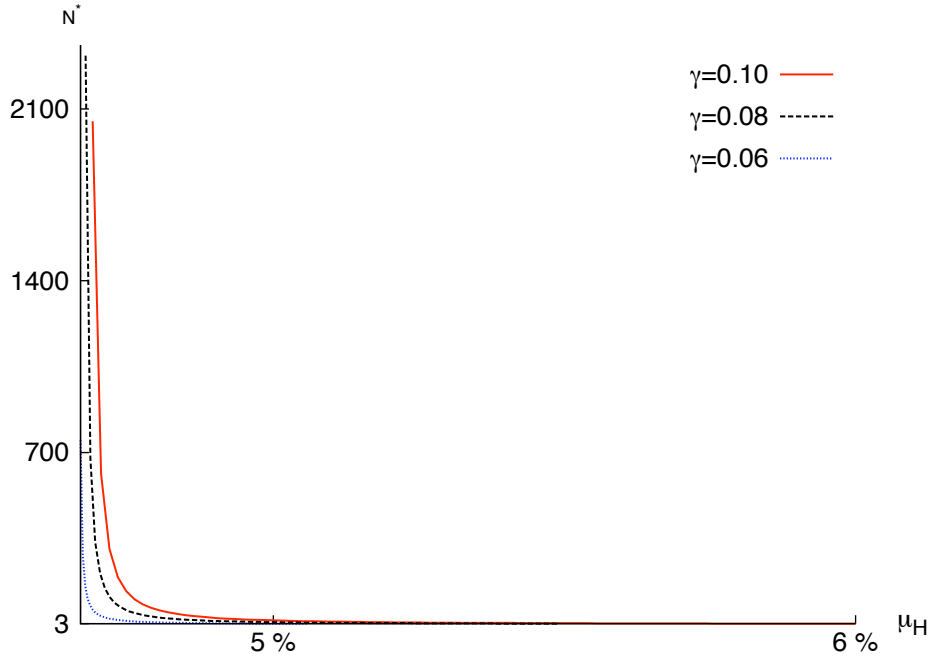
(b) N^* as a function of \mu_H
