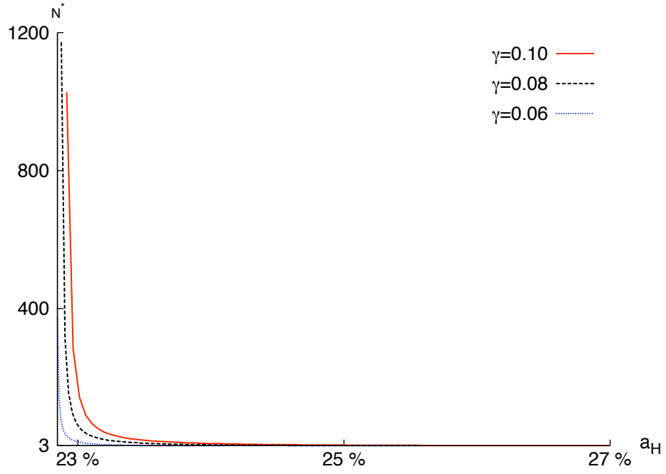
(a) N^* as a function of a_H
